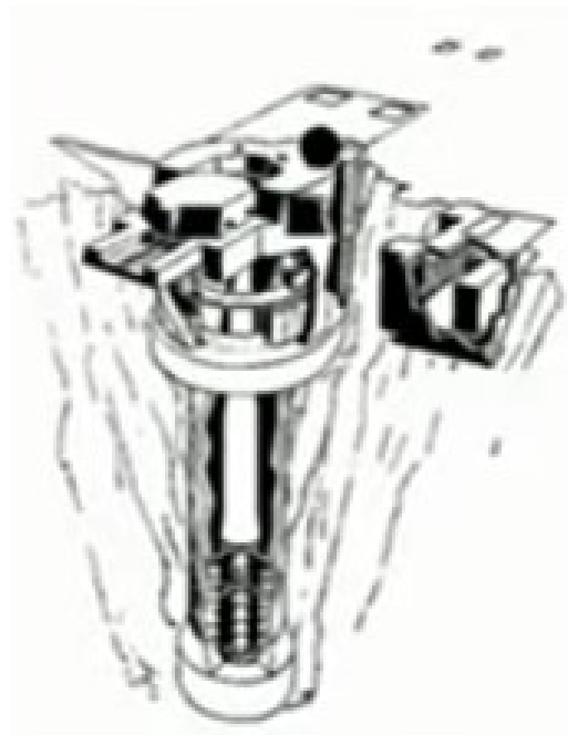
Fig 9.5 – A Cutaway Sketch Of The Underground Nuclear Missile Launch Facility
